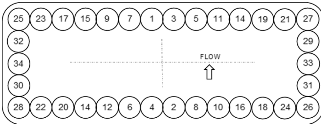
Figure 16: 18" 150-600
