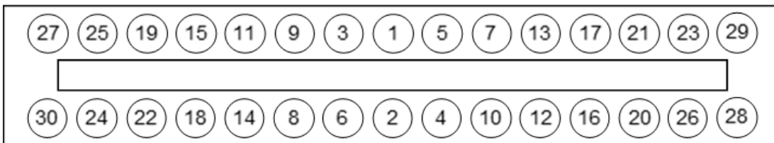
Figure 32: 34 Screw Pattern
