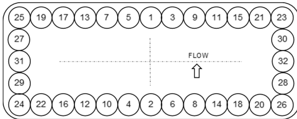
Figure 15: 16" 1500
